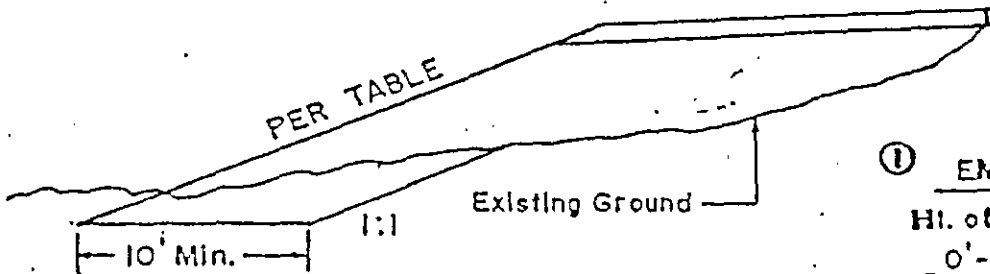
FILL TO BE CONSTRUCTED ON ROCK FOUNDATION
