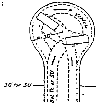
CIRCULAR-ALL PAVED
