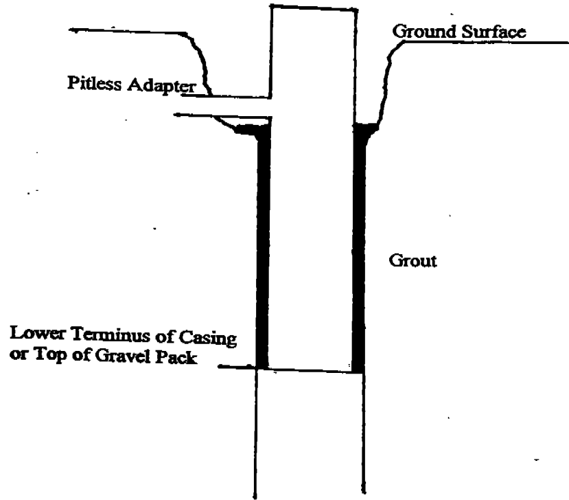
Figure 64-77 I Requirements for Grouting Wells with Pitless Adapters
