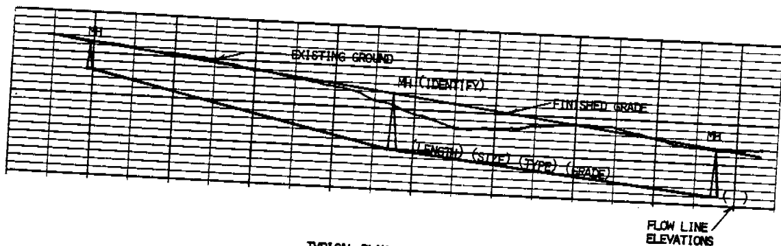
TYPICAL PLAN - PROFILE
