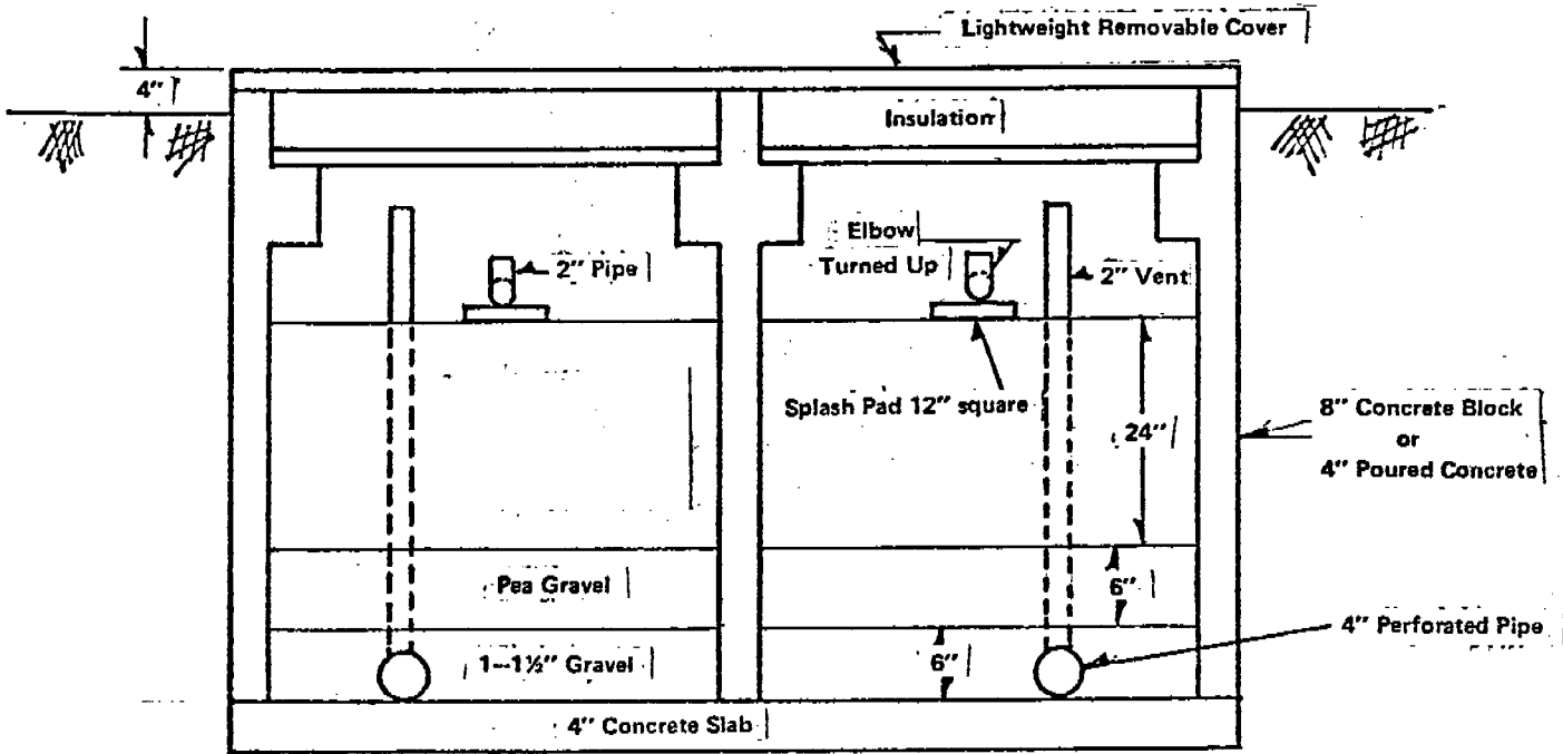
TYPICAL SURFACE SAND FILTERS
