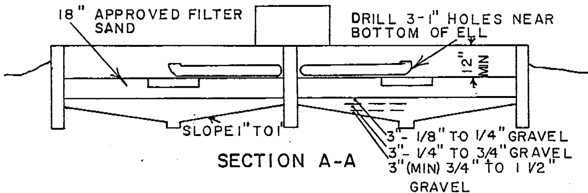
ALTERNATING SURFACE SAND FILTER DOSED BY FLOODING
