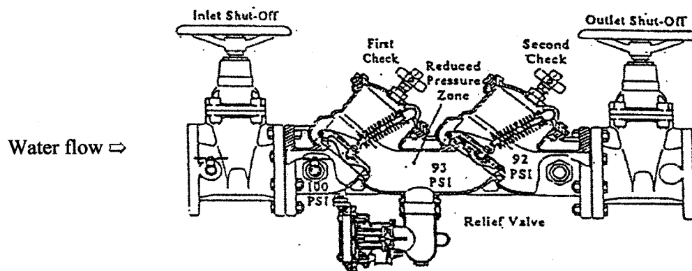
FIGURE 6 - Reduced Pressure Principle Backflow Preventer
