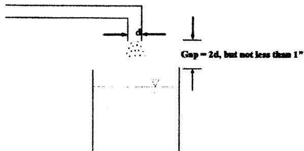
FIGURE 5 - Typical Air Gap
