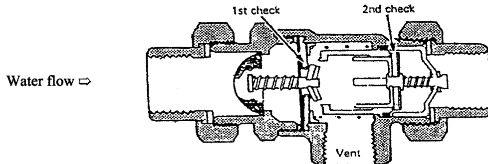
FIGURE 8- Double Check Valve with Intermediate Atmospheric Vent
