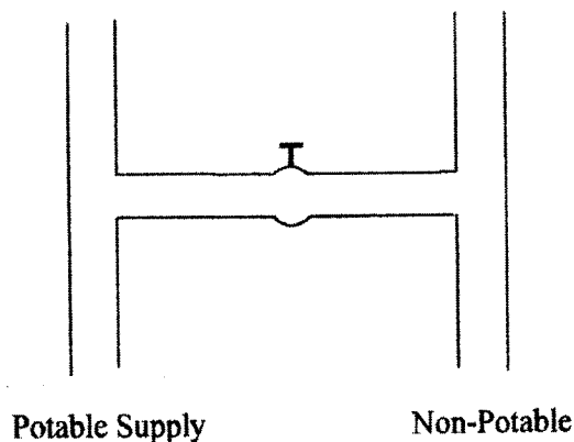
FIGURE 1 - Typical Direct Connection
