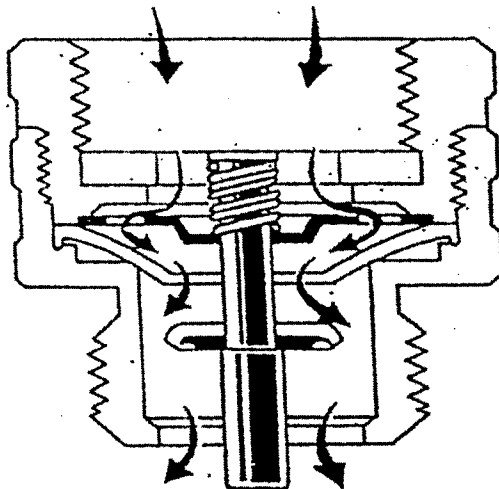
FIGURE 12 - Hose Bibb Vacuum Breaker
