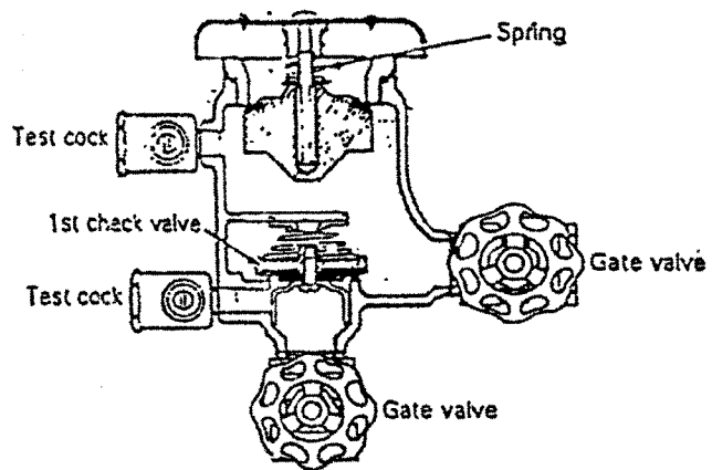
FIGURE 11 - Pressure Vacuum Breaker
