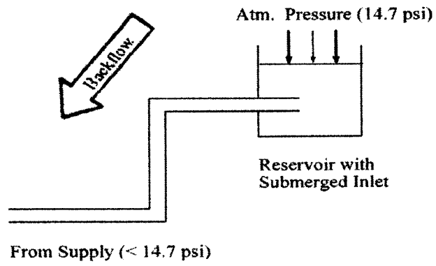
FIGURE 4 - Backsiphonage
