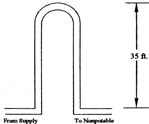
FIGURE 13 - Barometric Loop
