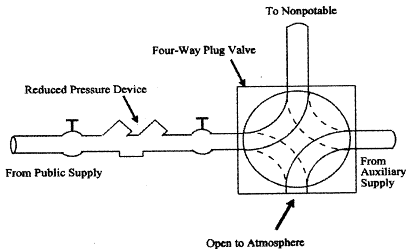
FIGURE 14 - Four-Way Plug Valve with Reduced Pressure Device
