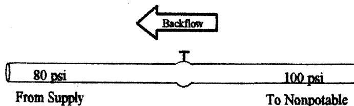
FIGURE 3 - Backflow due to Backpressure
