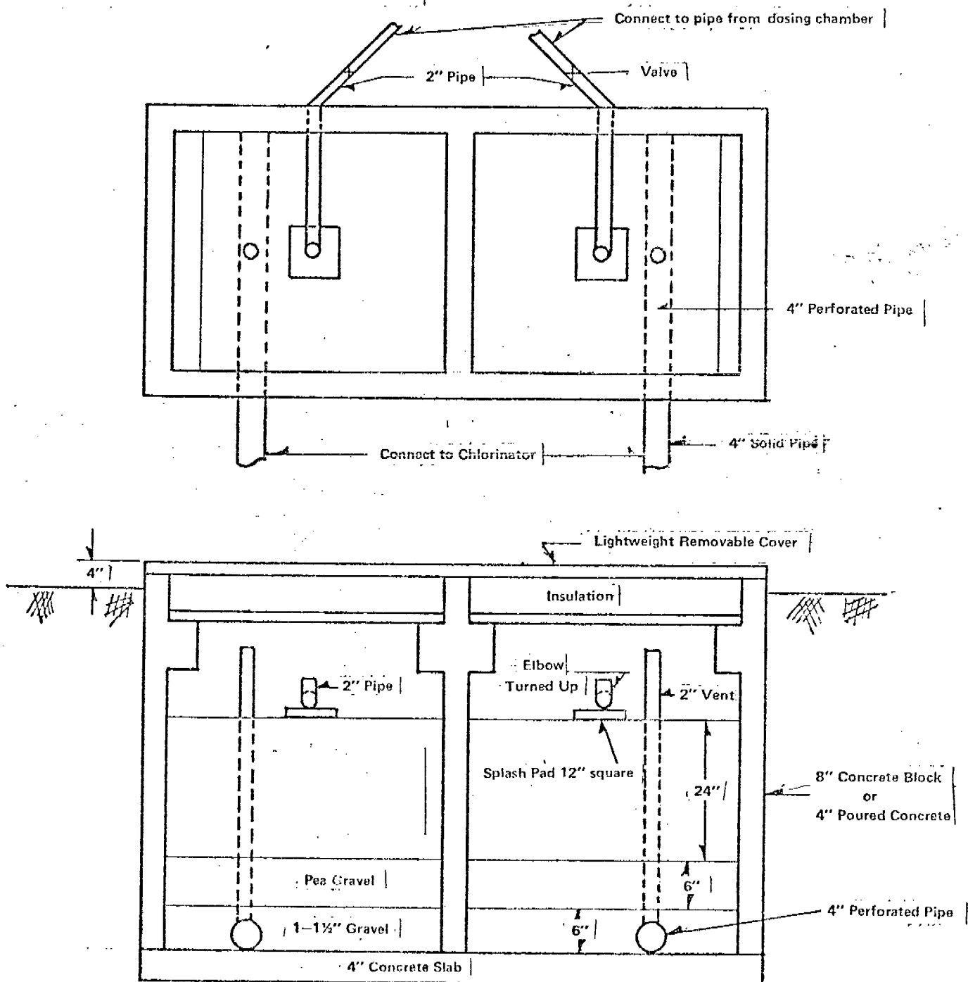
TYPICAL SURFACE SAND FILTERS
