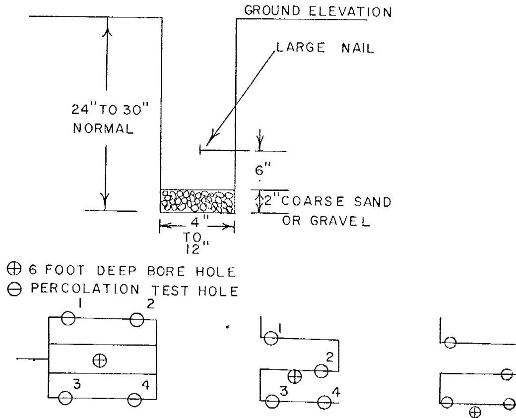
TYPICAL SPACING OF PERCOLATION TEST HOLES ON PROPOSED ABSORPTION FIELDS
