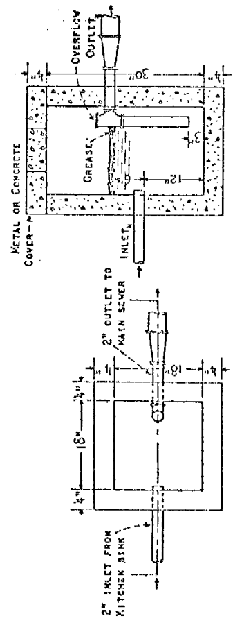
PLAN - COVER REMOVED GREASE TRAP SECTION
