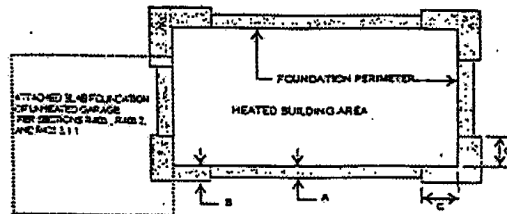
HORIZONTAL INSULATION PLAN
