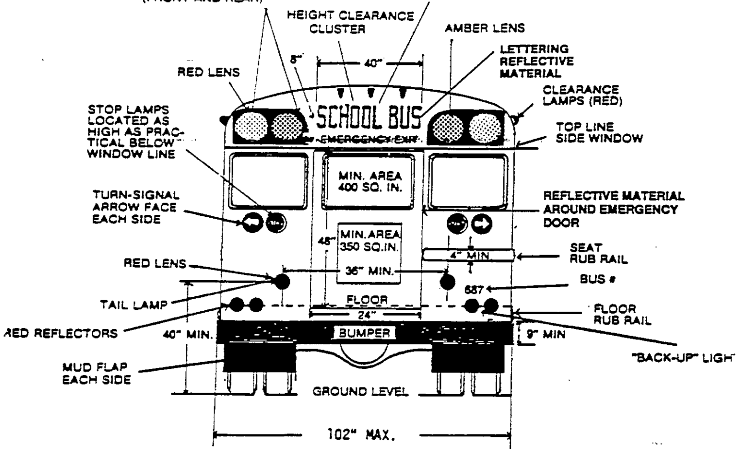
REAR ELEVATION
