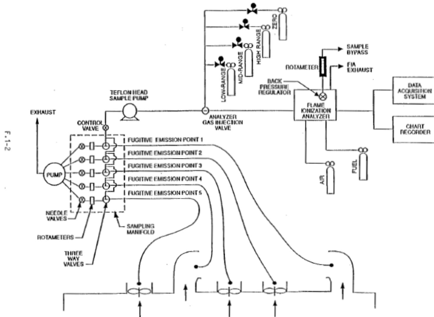
Figure F.1-1 Fugitive emissions measurement system.
