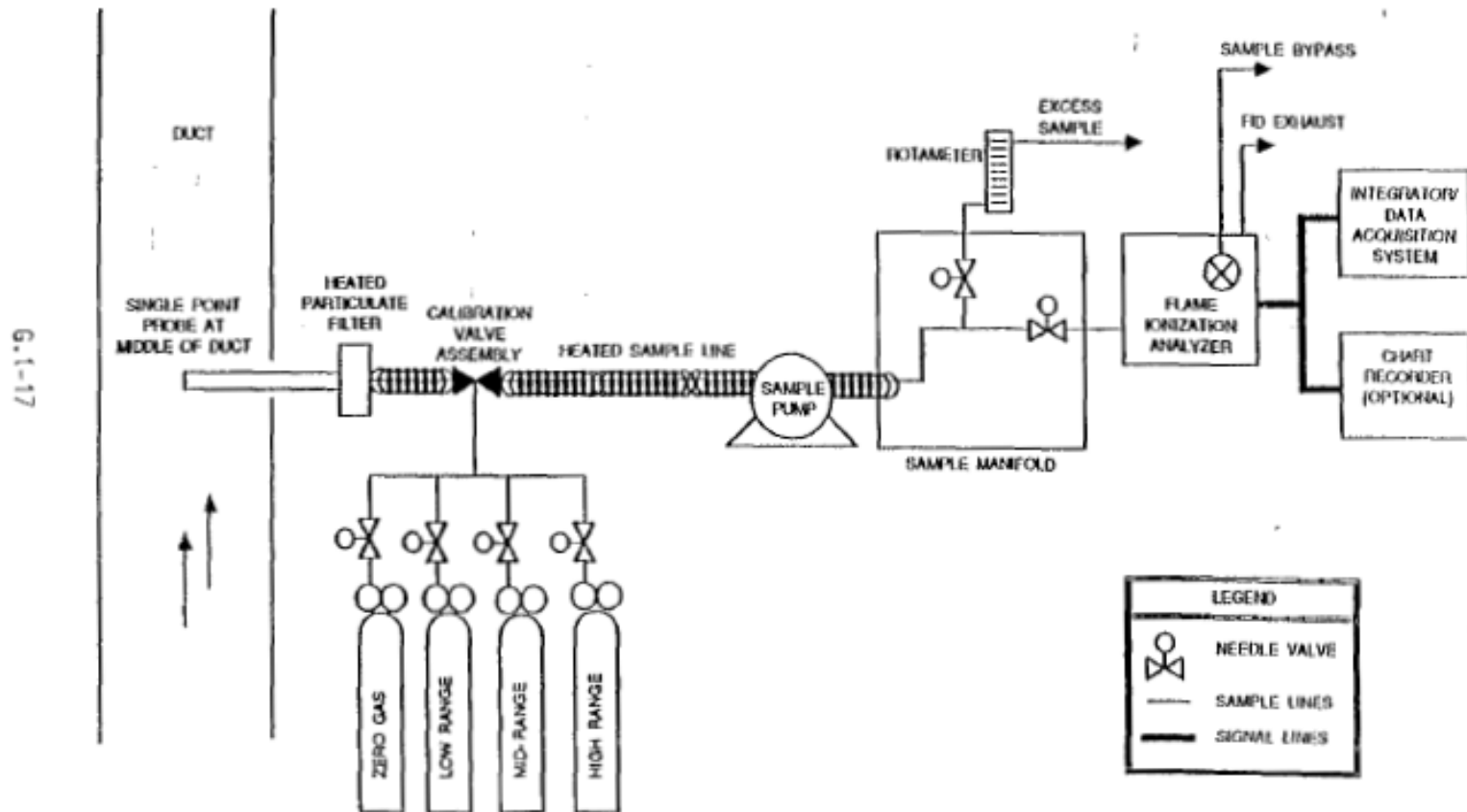
Figure G.1-1 Gas VOC concentration measurement system.
