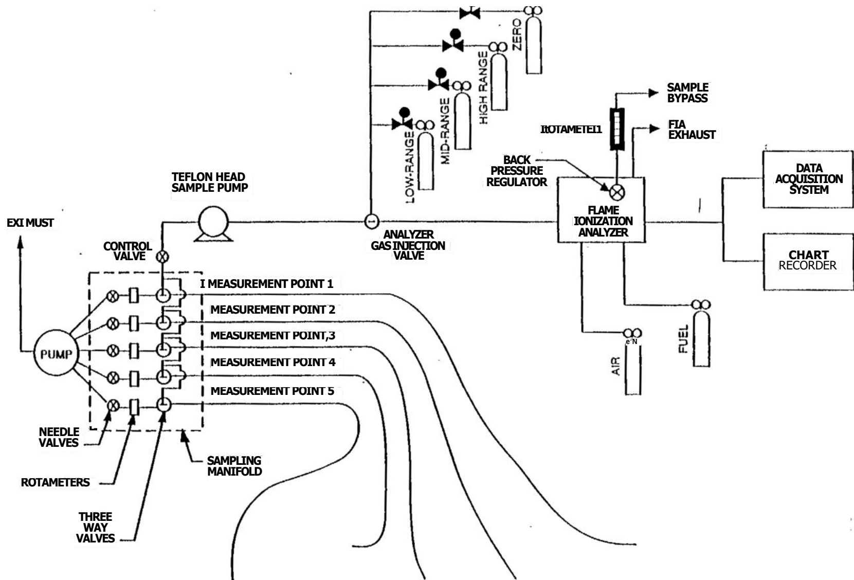
Figure G.1-2 Background measurement system.
