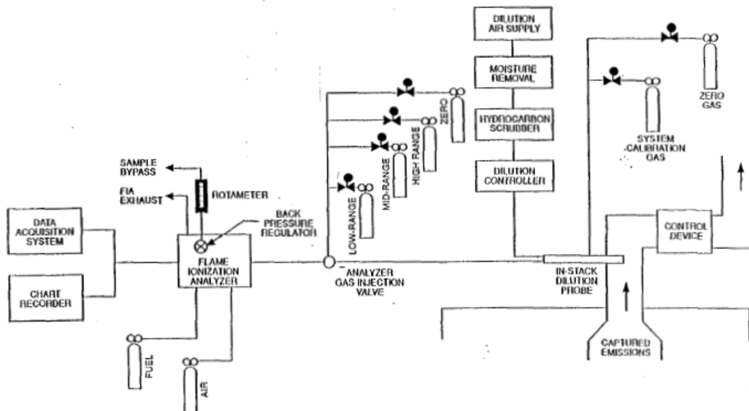
Figure G.2-1 Captured emissions measurement system.
