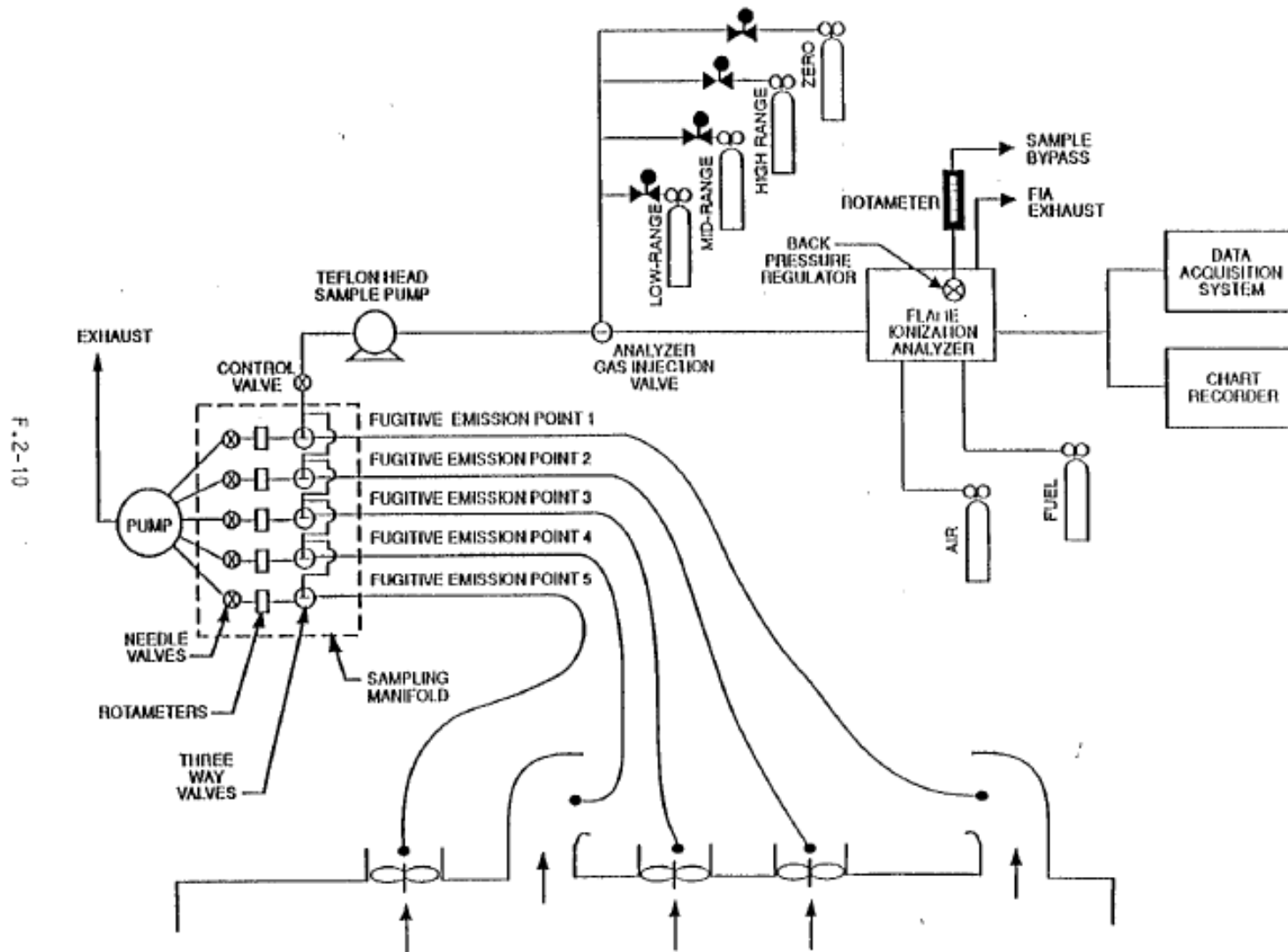
Figure F.2-1 Fugitive emissions measurement system.
