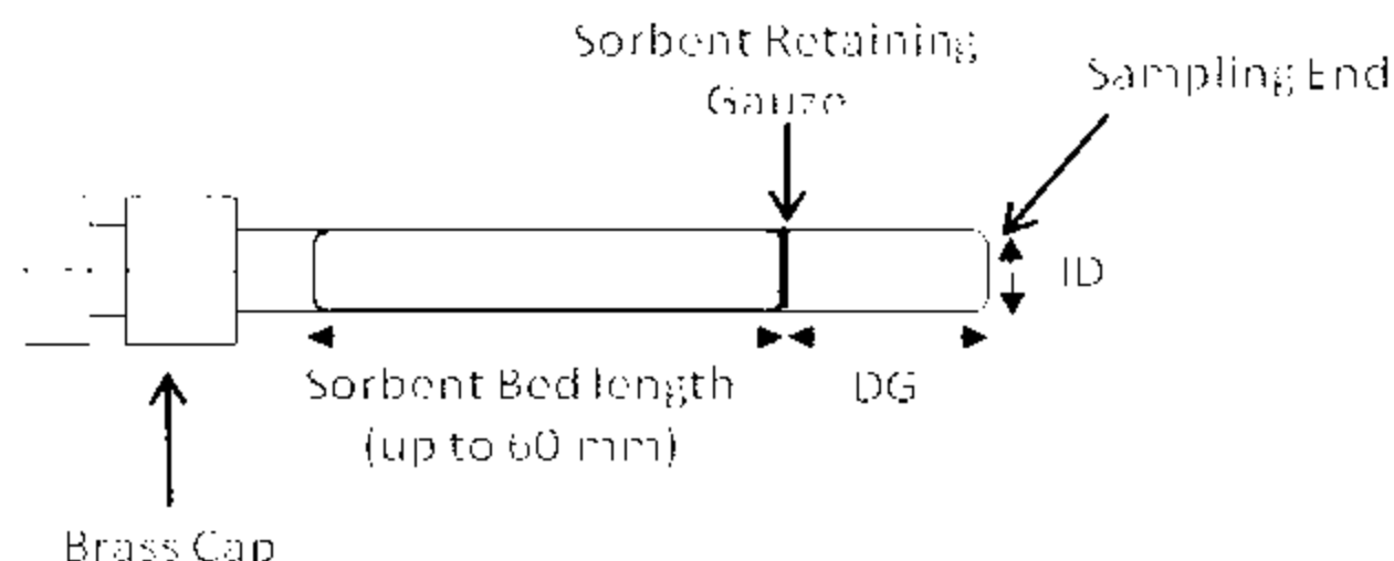
Figure 6.1. Cross Section View of Passive Sorbent Tube
