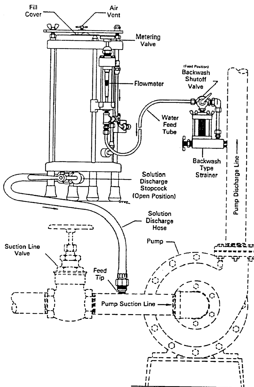
Figure 29. Suction Feeder
