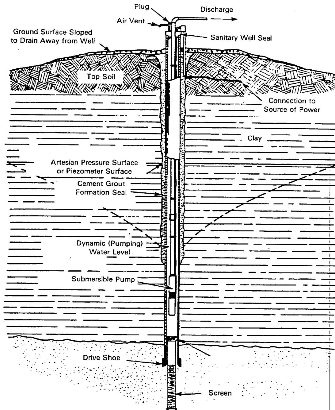
Figure 14. Drilled Well with Submersible Pump
