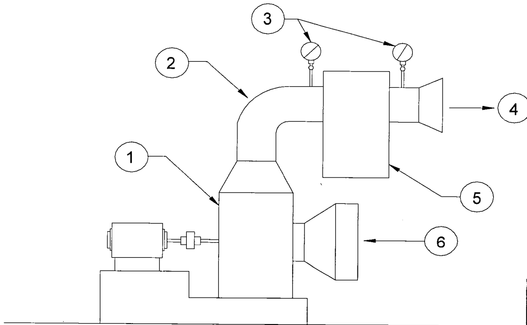
Figure 46. Individual Blower-Type Air Supply
