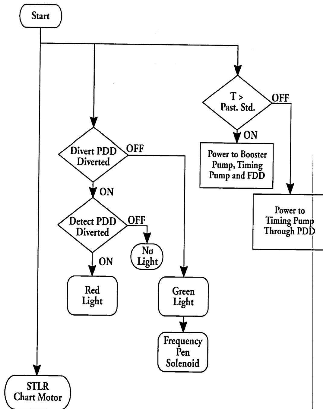
Figure 54. Logic Diagram: HTST Safety Thermal Limit Recorder-Controller
