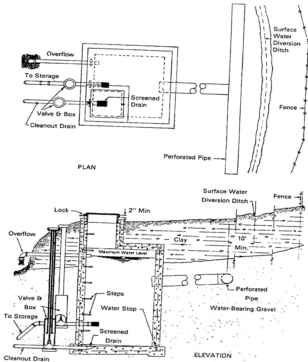
Figure 17. Spring Protection
