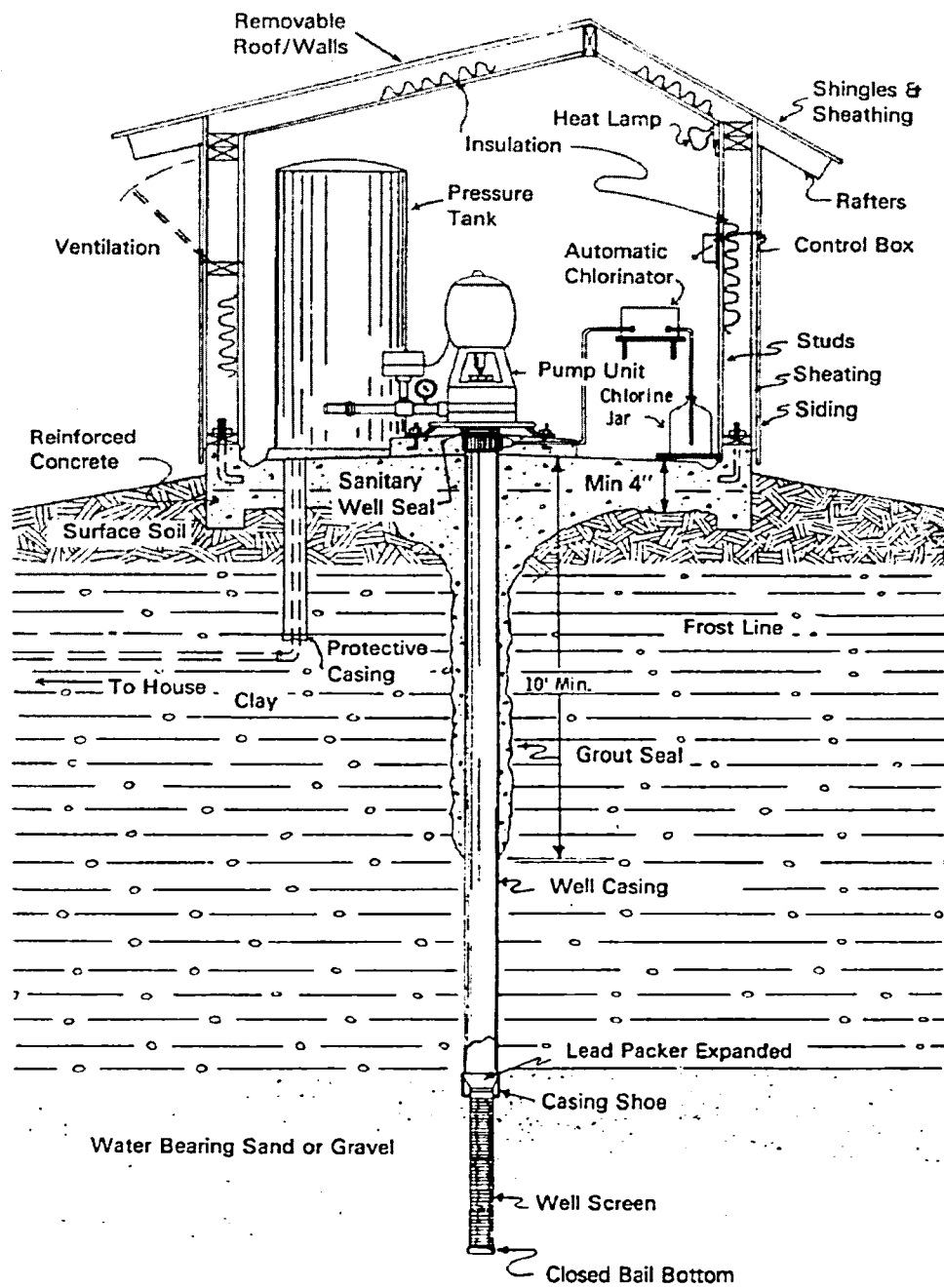
Figure 16. Pumphouse
