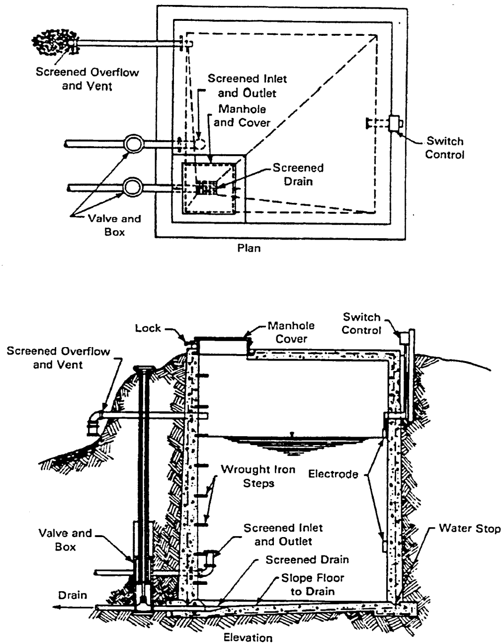
Figure 21. Typical Concrete Reservoir
