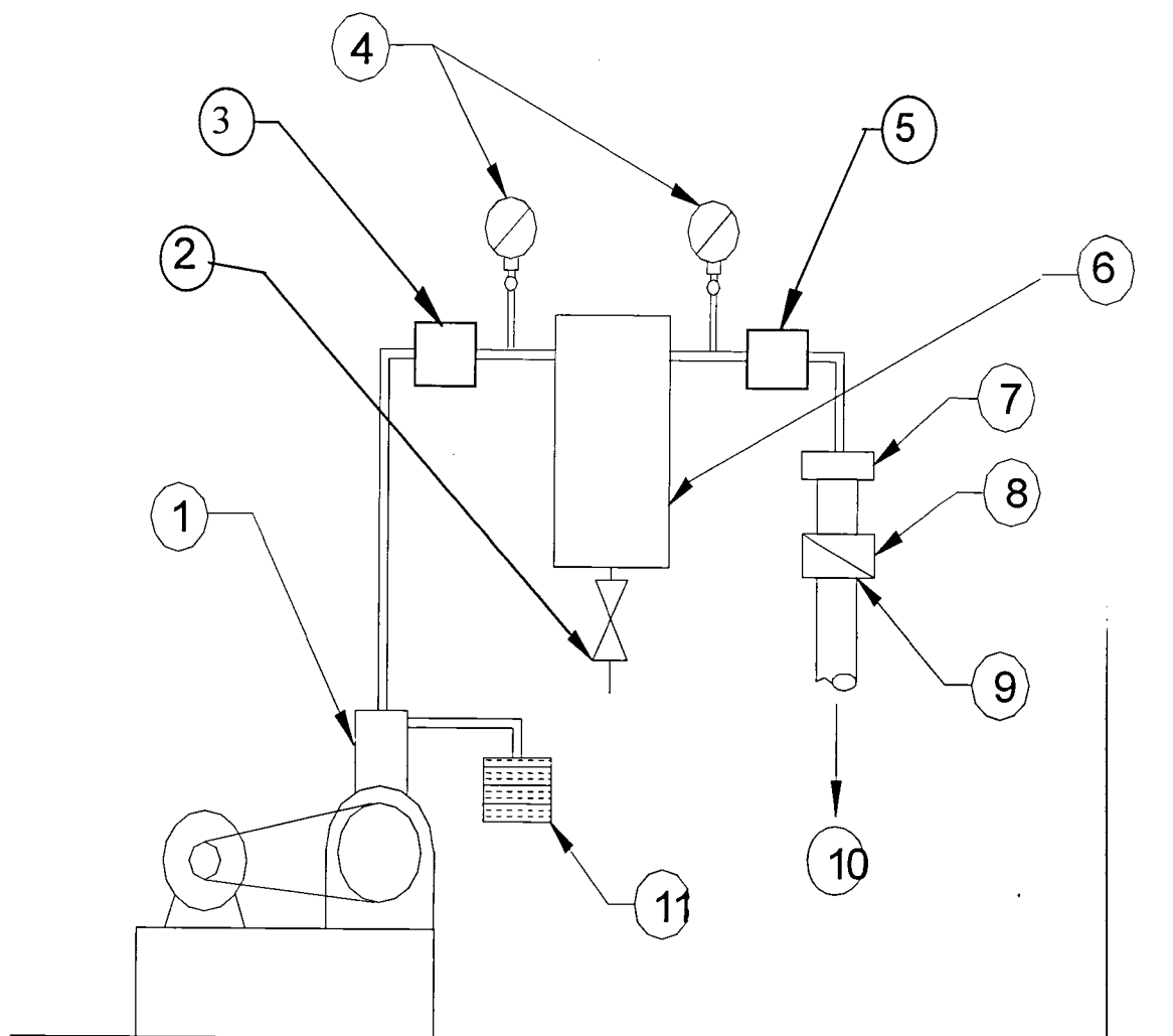
Figure 44. Individual Compression-Type Air Supply
