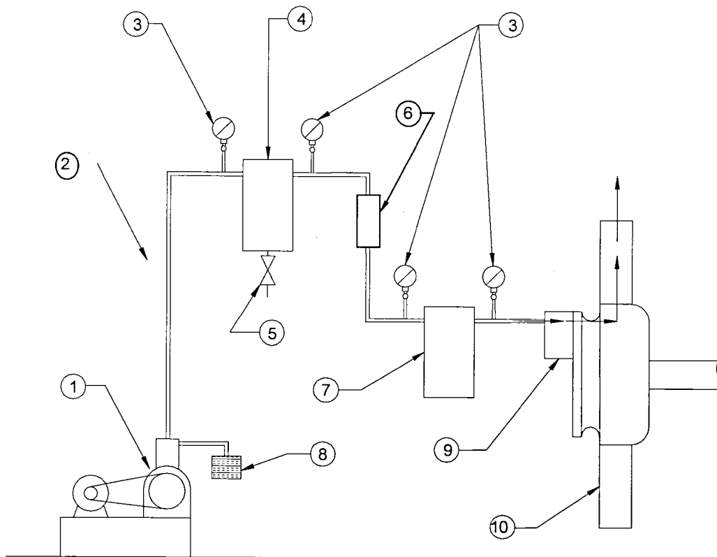
Figure 48. Rotating Mandrel Assembly
