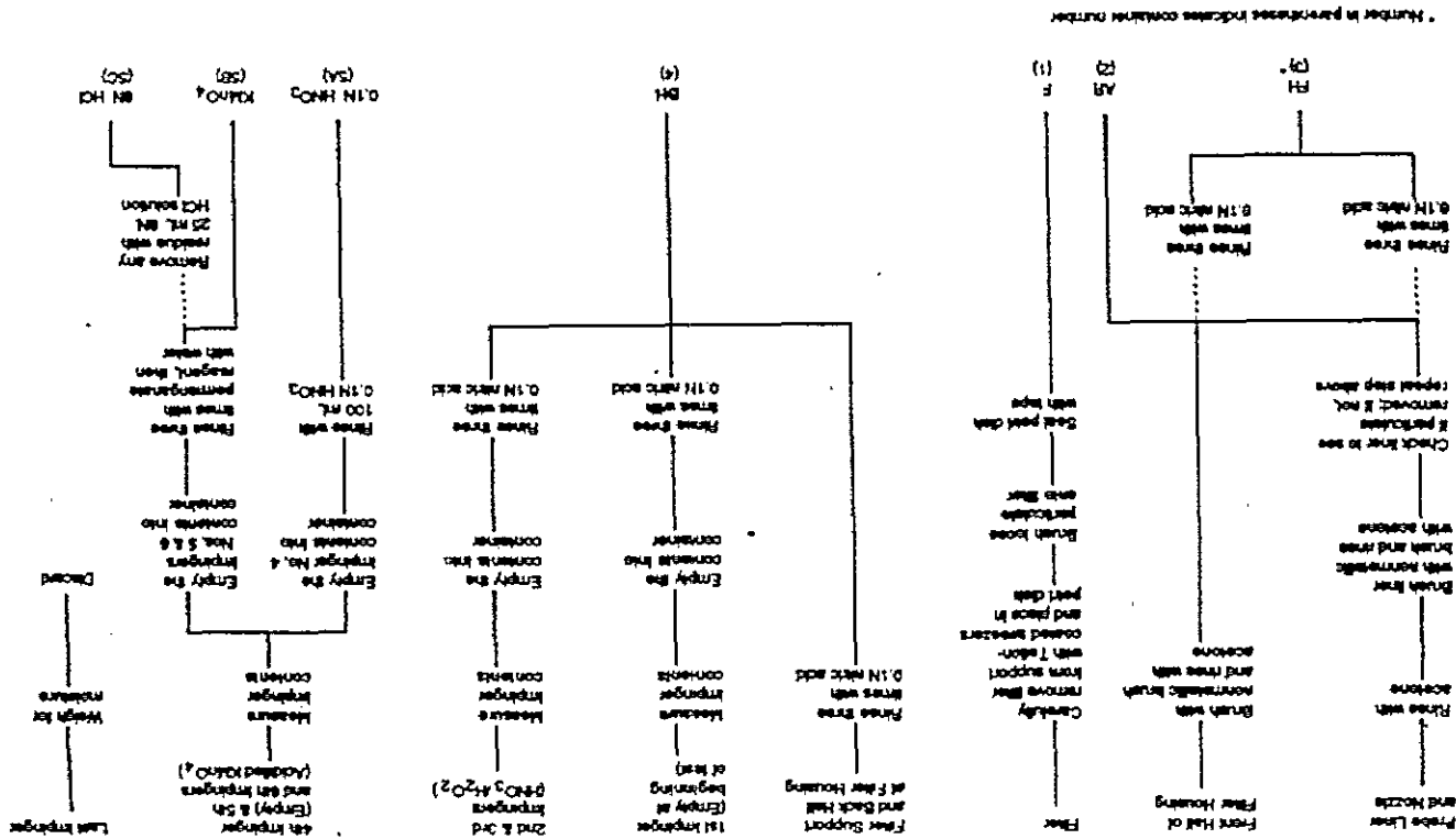
Figure 3.1-2 Sample recovery scheme.
