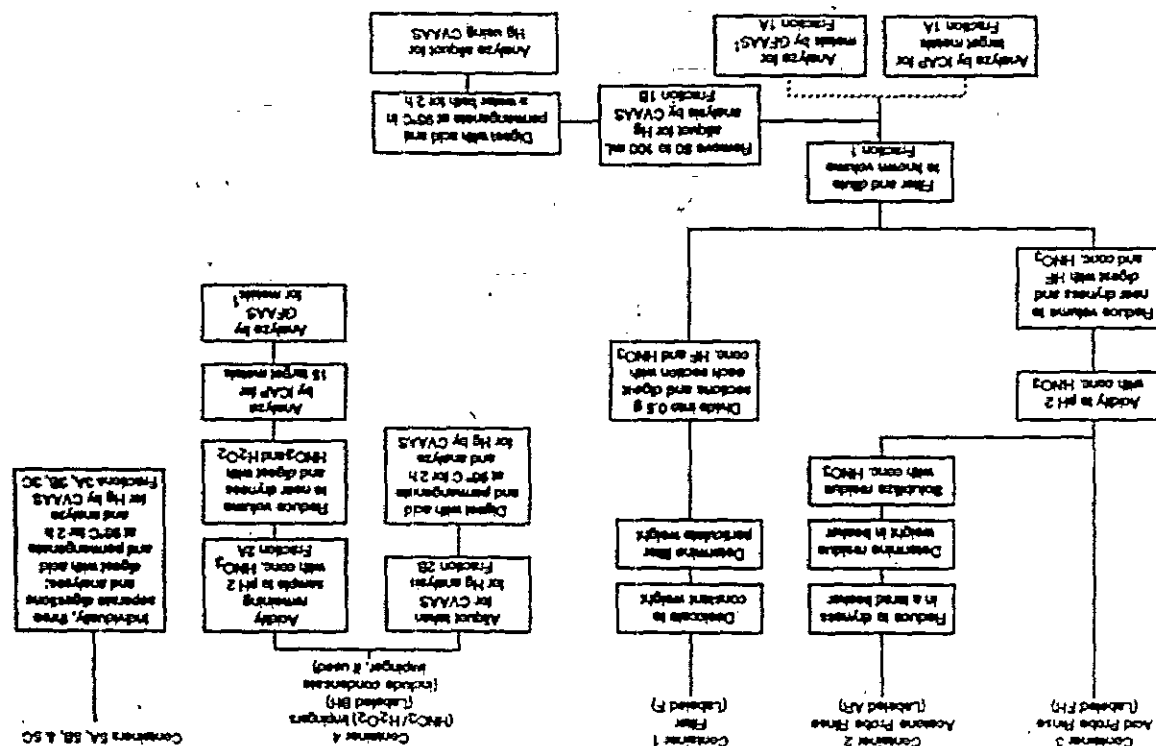
Figure 3.1-3 Sample preparation and analysis scheme.
