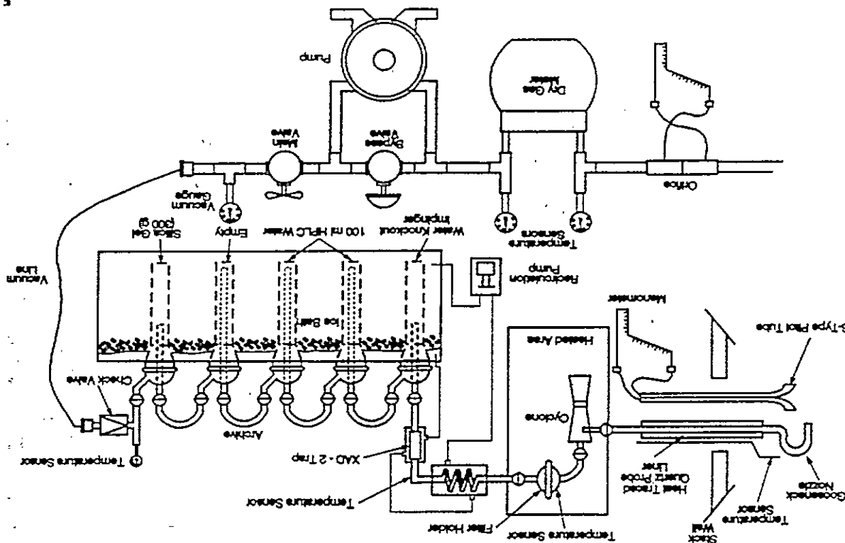
Figure 3.4-1 Sampling Train
