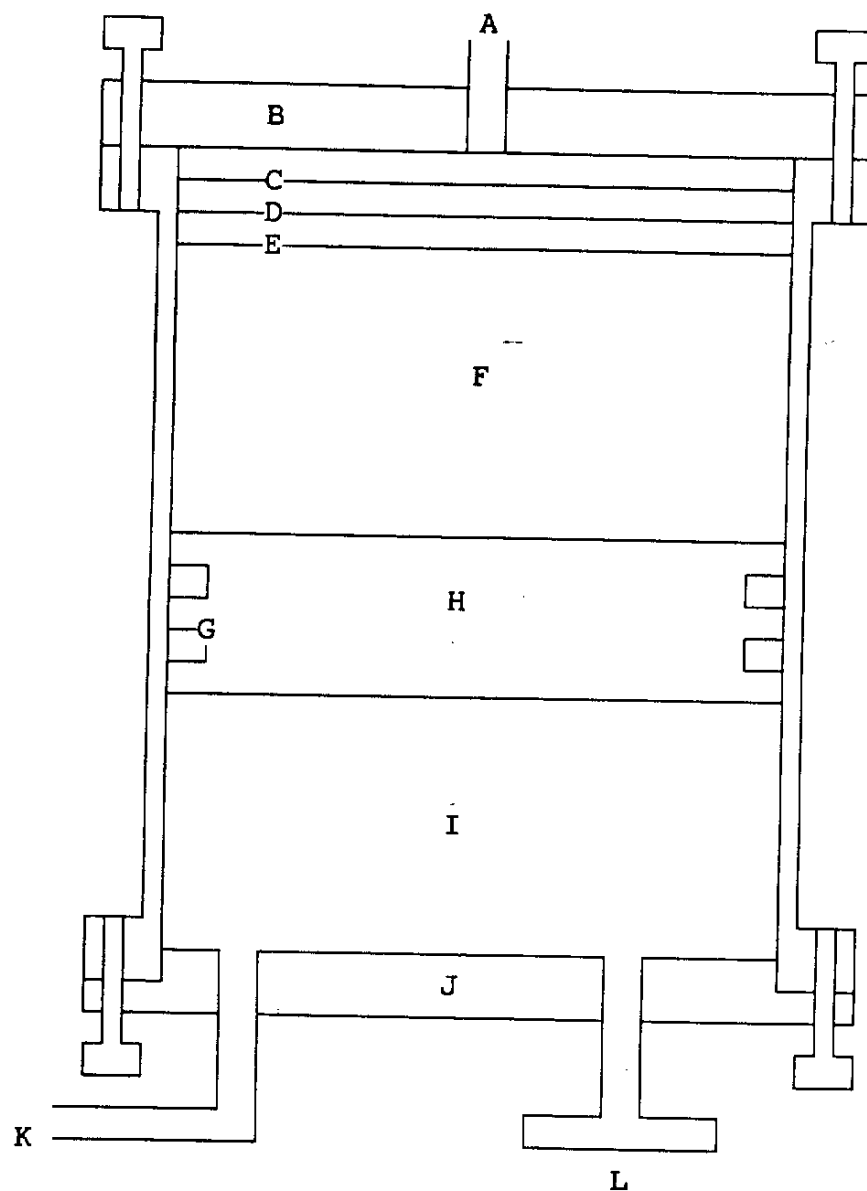
FIGURE 2. -- ZERO HEADSPACE EXTRACTOR
