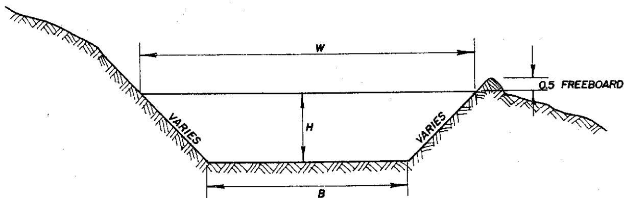
TRAPEZOIDAL
