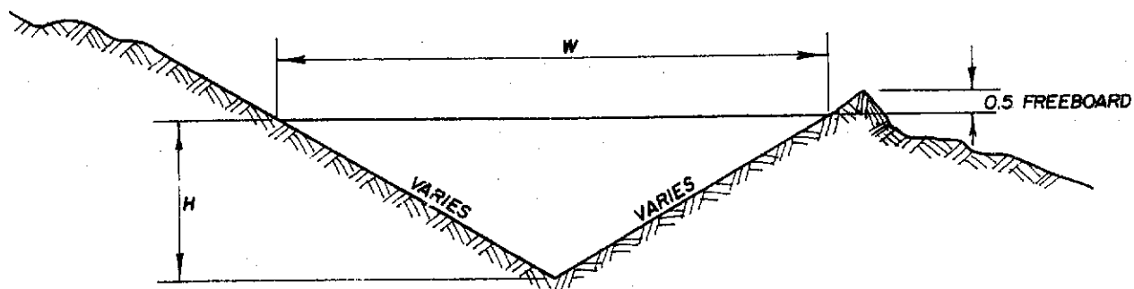
TRIANGULAR
