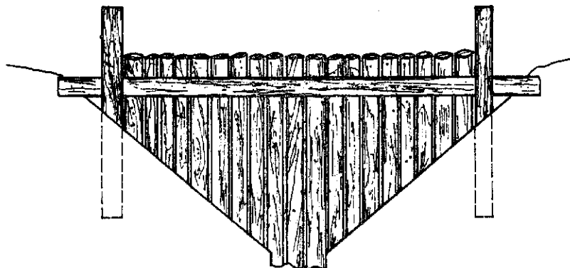
UPSTREAM VIEW
