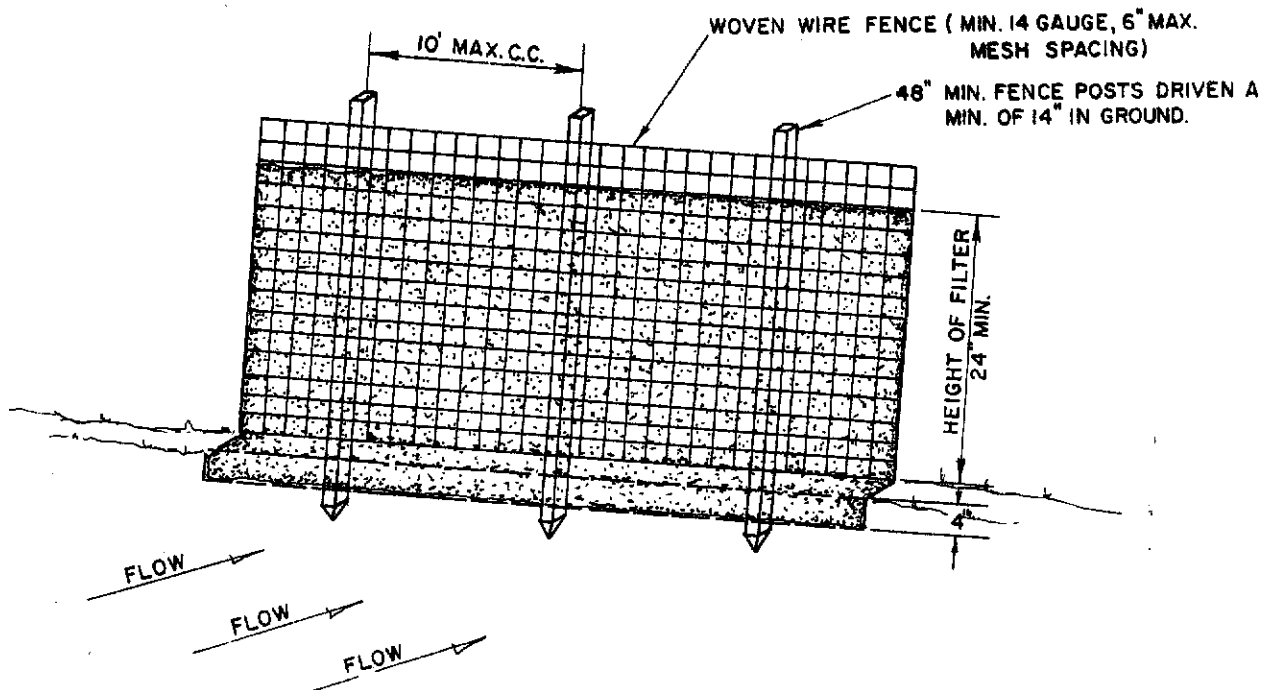
PERSPECTIVE VIEW
