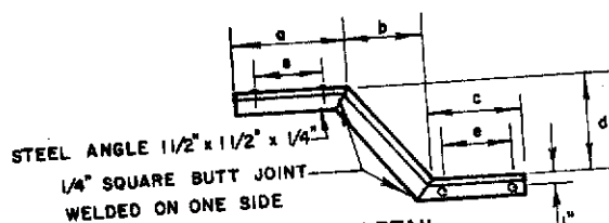
(1 LEFT AND 1 RIGHT REQUIRED EACH BAFFLE)
