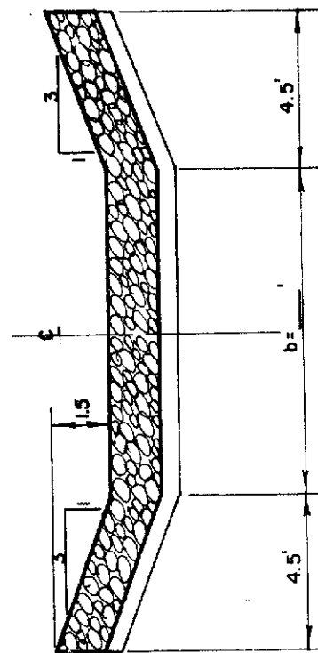
CHUTE SECTION
