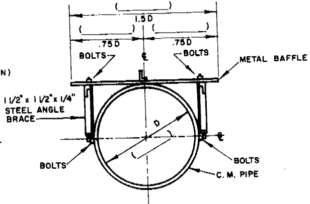
FRONT ELEVATION
