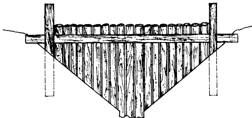
UPSTREAM VIEW
