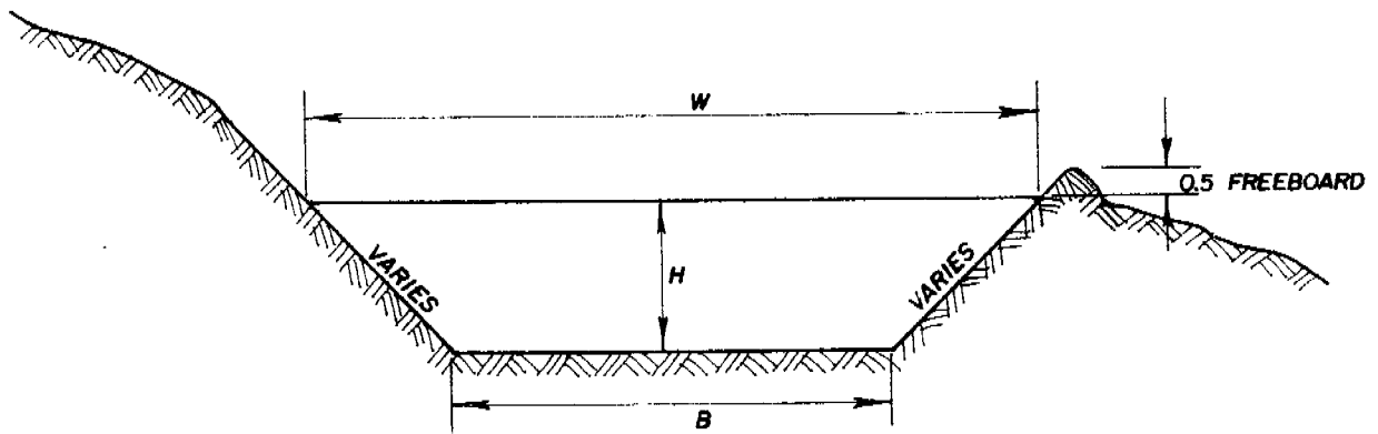
TRAPEZOIDAL
