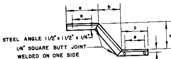
ANGLE BRACE DETAIL
