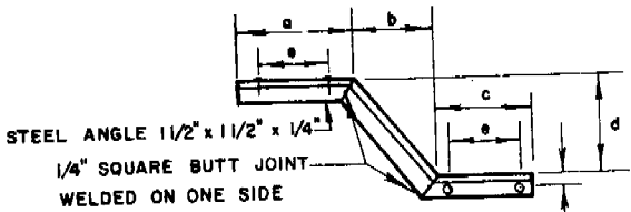
ANGLE BRACE DETAIL (1 LEFT AND 1 RIGHT REQUIRED EACH BAFFLE)
