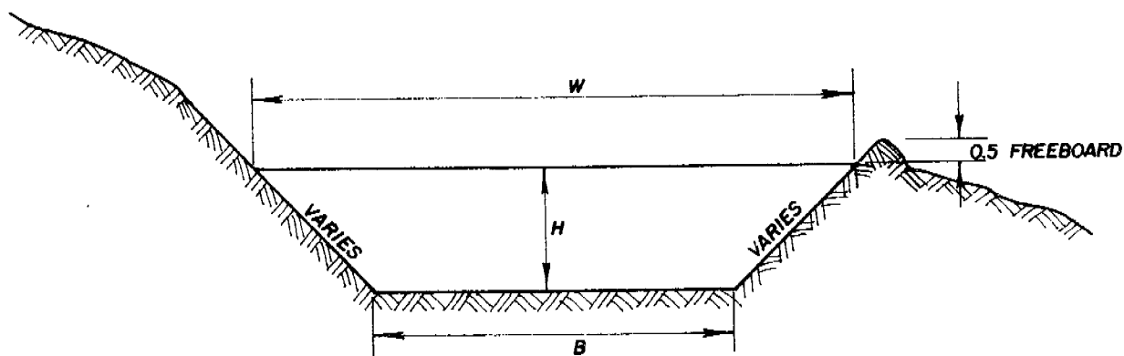
TRAPEZOIDAL
