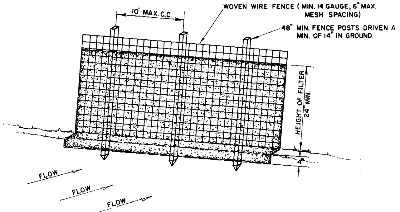
PERSPECTIVE VIEW
