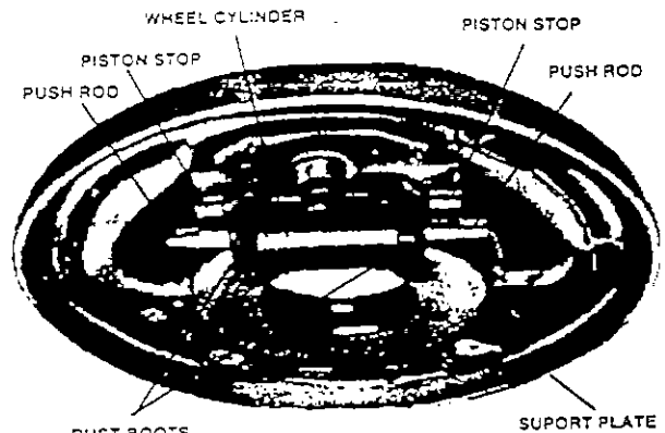
TYPICAL DRUM-BRAKE BACKING PLATE with most parts removed, showing wheel cylinder and dust boots.
