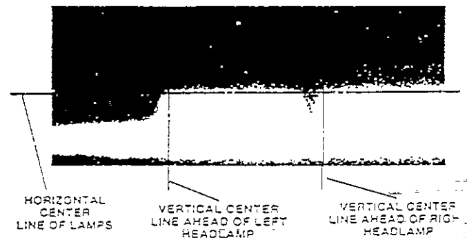
CORRECT AIM ADJUSTMENT FOR LOW BEAM
