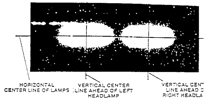
CORRECT AIM ADJUSTMENT FOR HIGH BEAM
