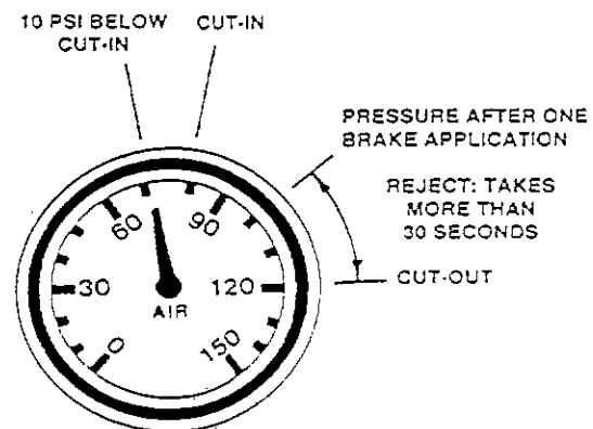
AIR GAUGE EXAMPLE READINGS FOR CHECKING AIR PRESSURE BUILDUP TIME
