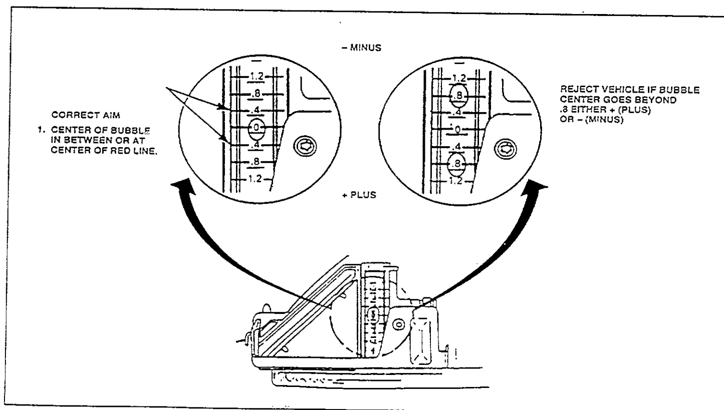
VHAD VERTICAL AIM
