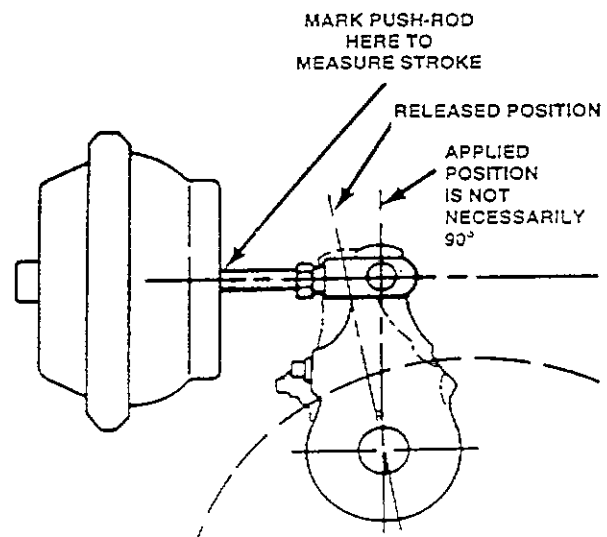
MEASURING THE CAM BRAKE ADJUSTMENT
