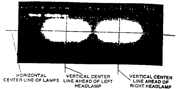
CORRECT AIM ADJUSTMENT FOR UPPER BEAM
