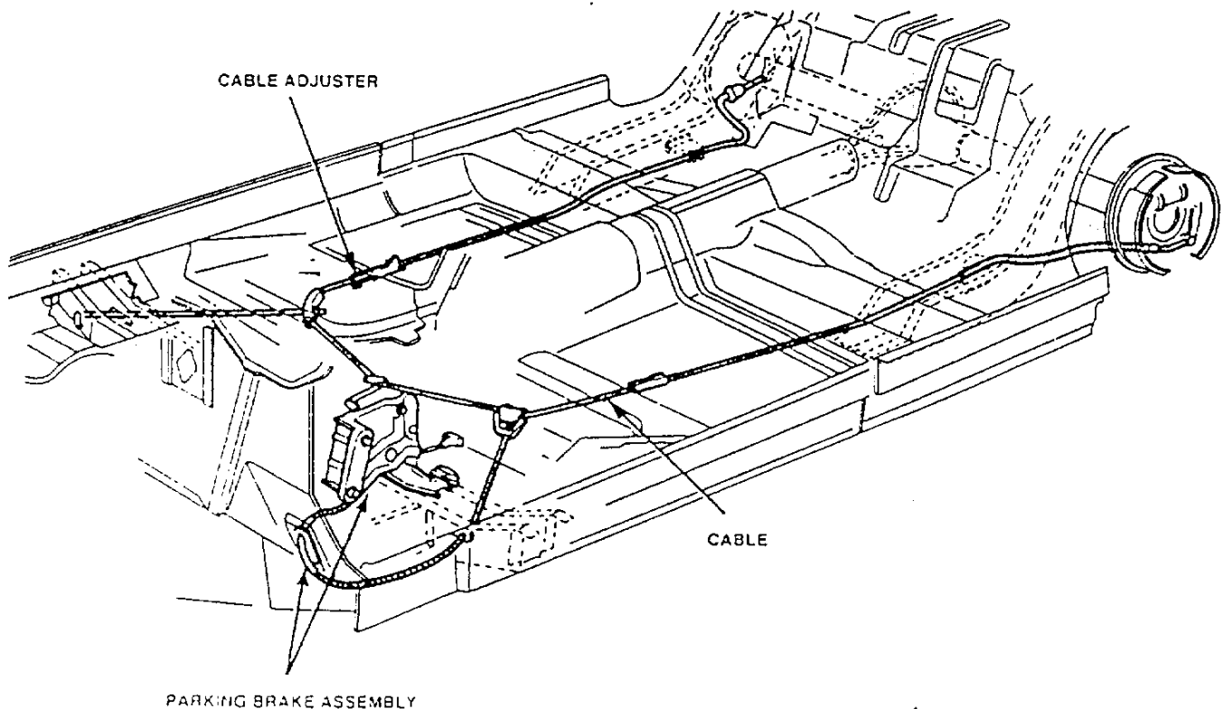
A TYPICAL PARKING BRAKE SYSTEM
