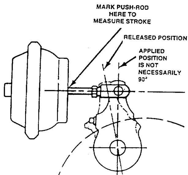
MEASURING THE CAM BRAKE ADJUSTMENT
