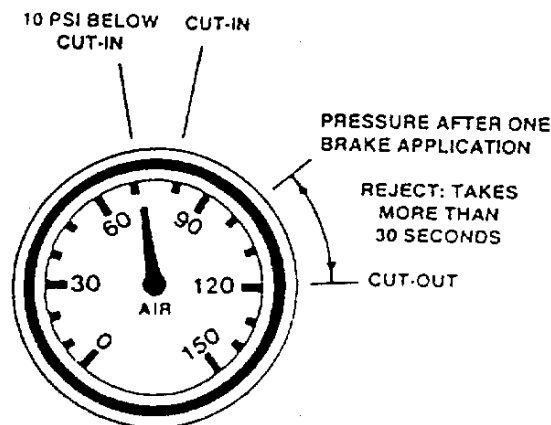
AIR GAUGE EXAMPLE READINGS FOR CHECKING AIR PRESSURE BUILDUP TIME
