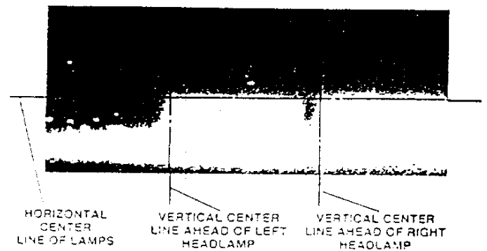
CORRECT AIM ADJUSTMENT FOR LOW BEAM
