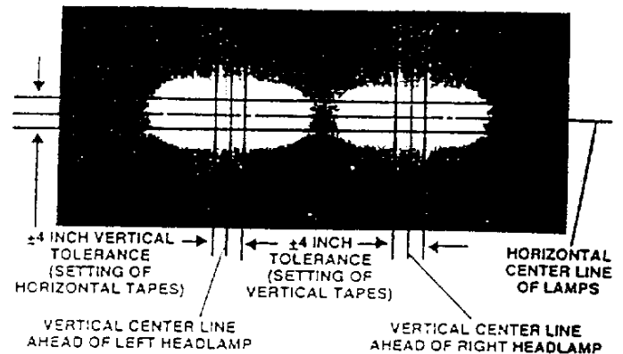
CORRECT AIM ADJUSTMENT FOR UPPER BEAM
