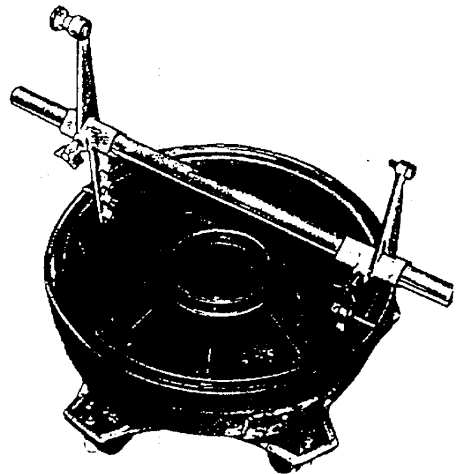
MEASURING INSIDE DIAMETER OF DRUM
